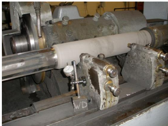
Splined Mandrel Coated In 1086 (Wc, Co, Cr)
