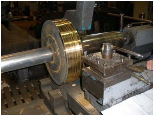
Operating piston with bronze overlay
